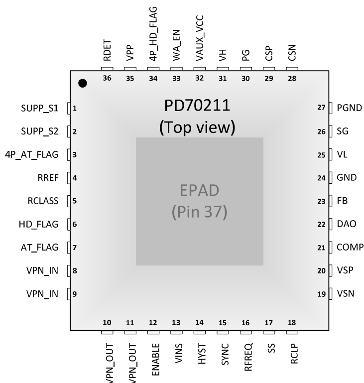
Figure 2: Pinout of PD70211 (top view)
