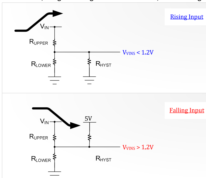
Figure 5: Equivalent Diagrams for UVLO and Hysteresis
