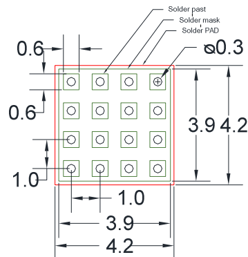
Figure 11: PD70224 Bottom layer Copper and Solder Paste Recommended PCB Layout for Thermal Pad Array (mm)
